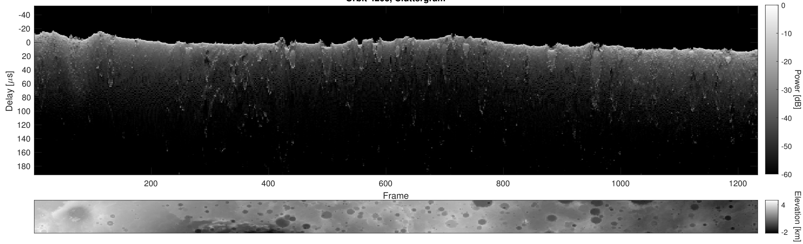
Orbit 4203, Cluttergram
