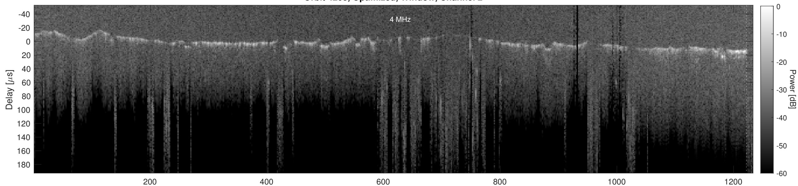
Orbit 4203, Cluttergram
