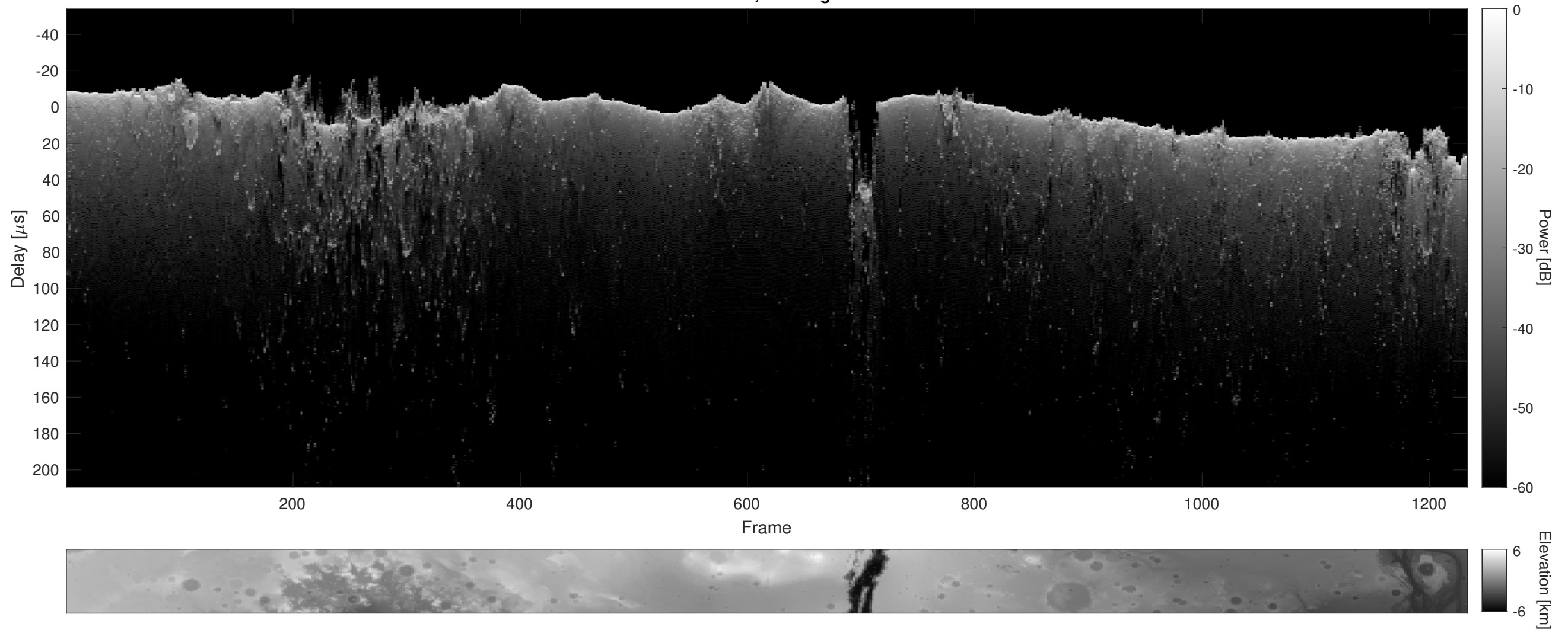
Orbit 4204, Cluttergram
