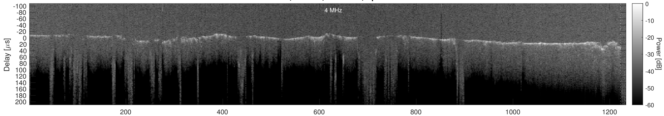
Orbit 4204, Cluttergram
