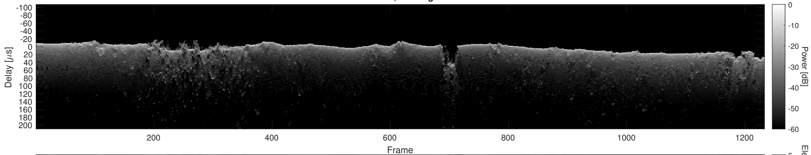
Orbit 4204, Cluttergram
