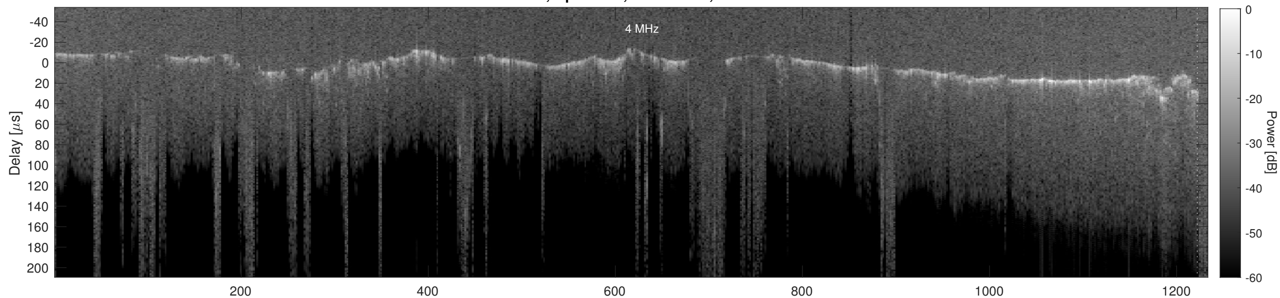
Orbit 4204, Cluttergram
