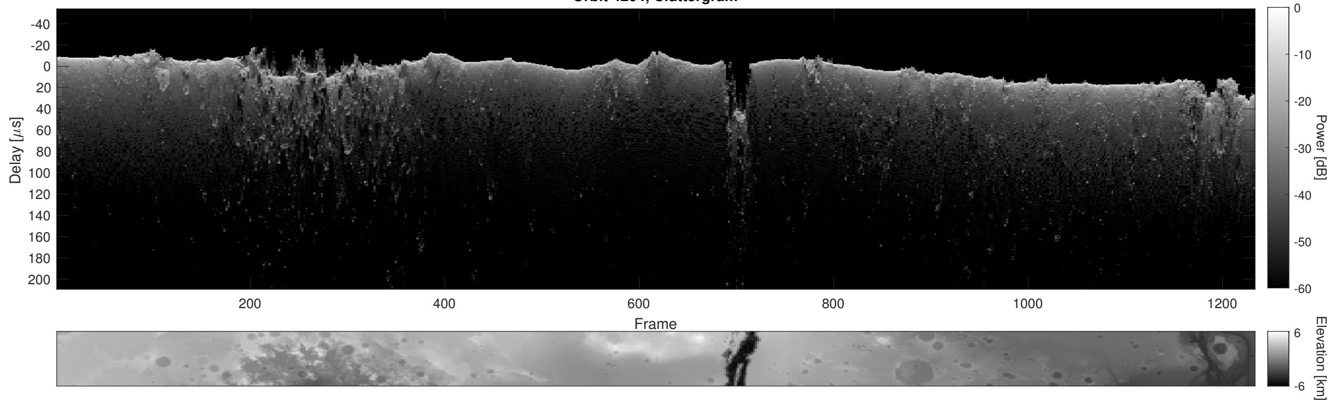
Orbit 4204, Cluttergram
