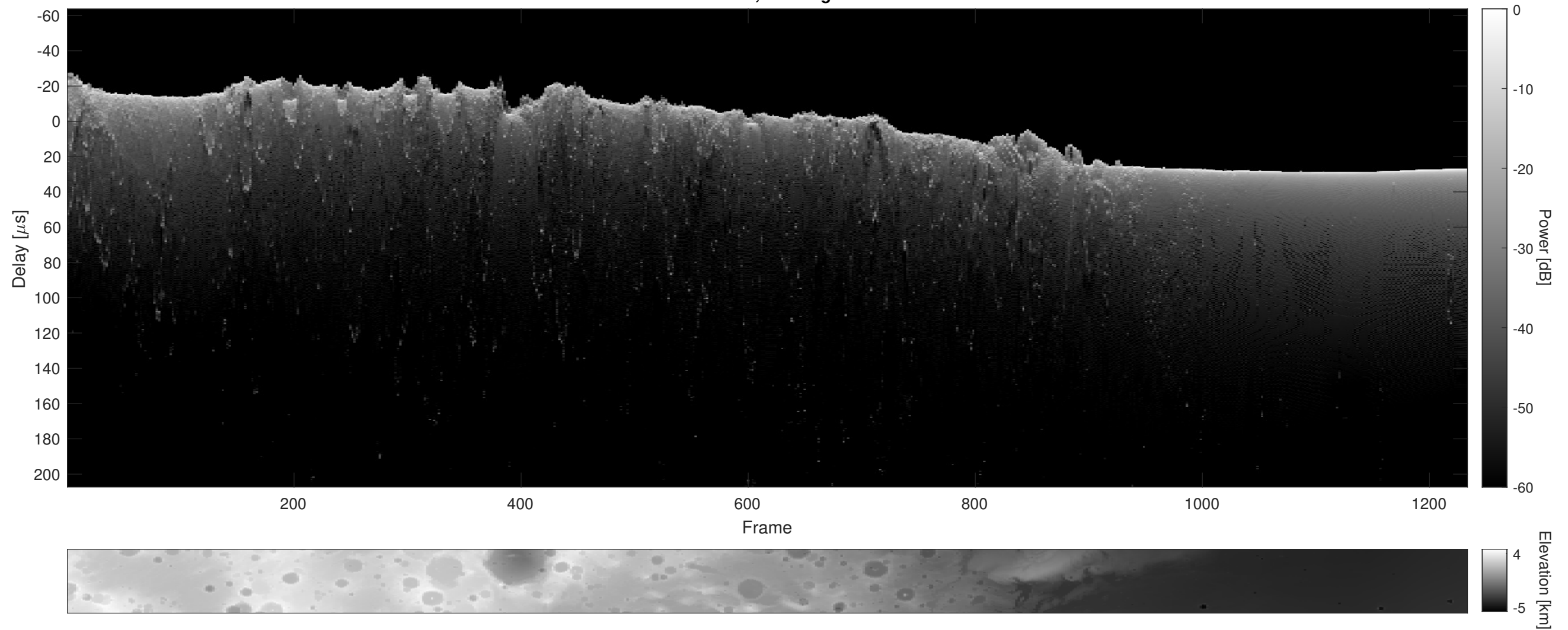
Orbit 4205, Cluttergram
