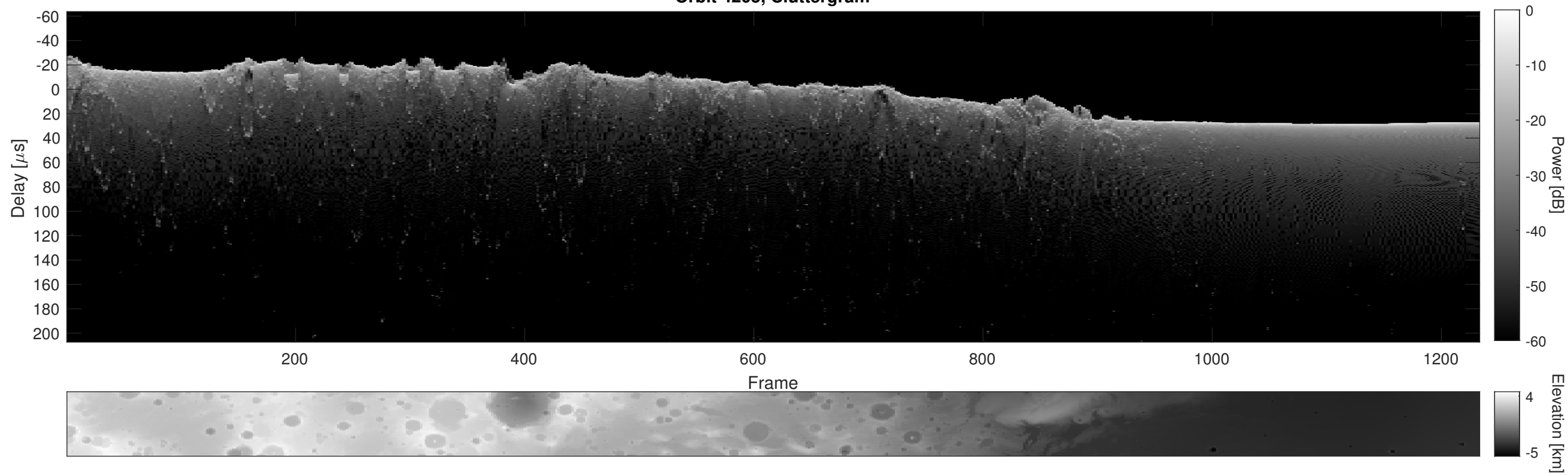
Orbit 4205, Cluttergram
