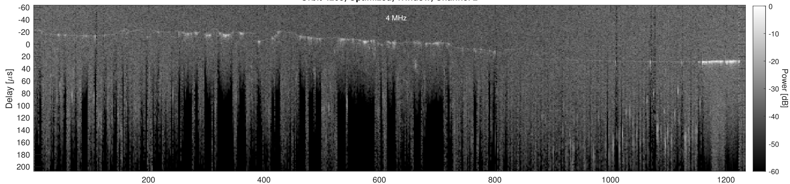
Orbit 4205, Cluttergram
