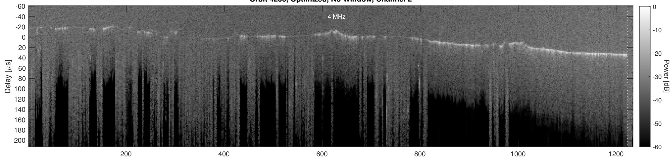
Orbit 4206, Cluttergram
