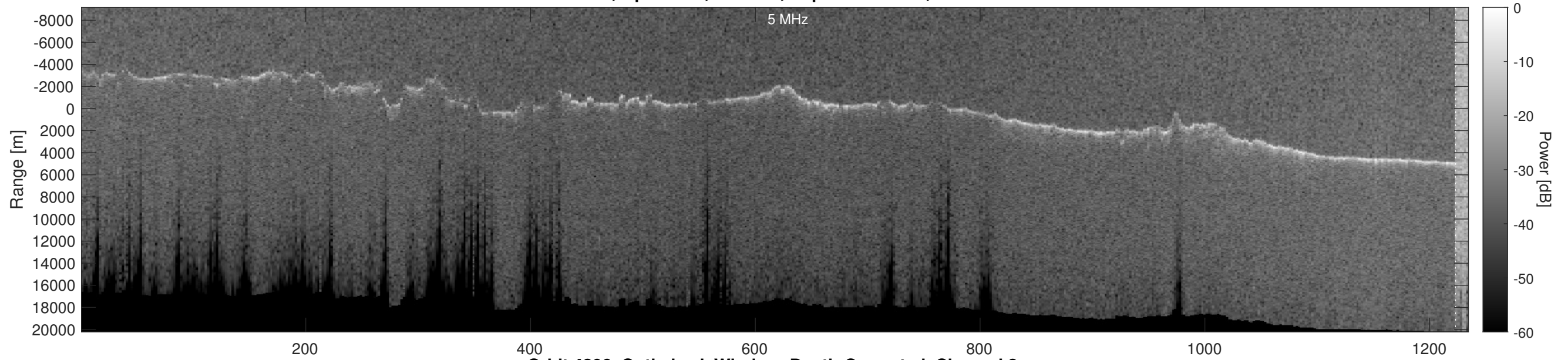
Orbit 4206, Optimized, Window, Depth-Corrected, Channel 2
