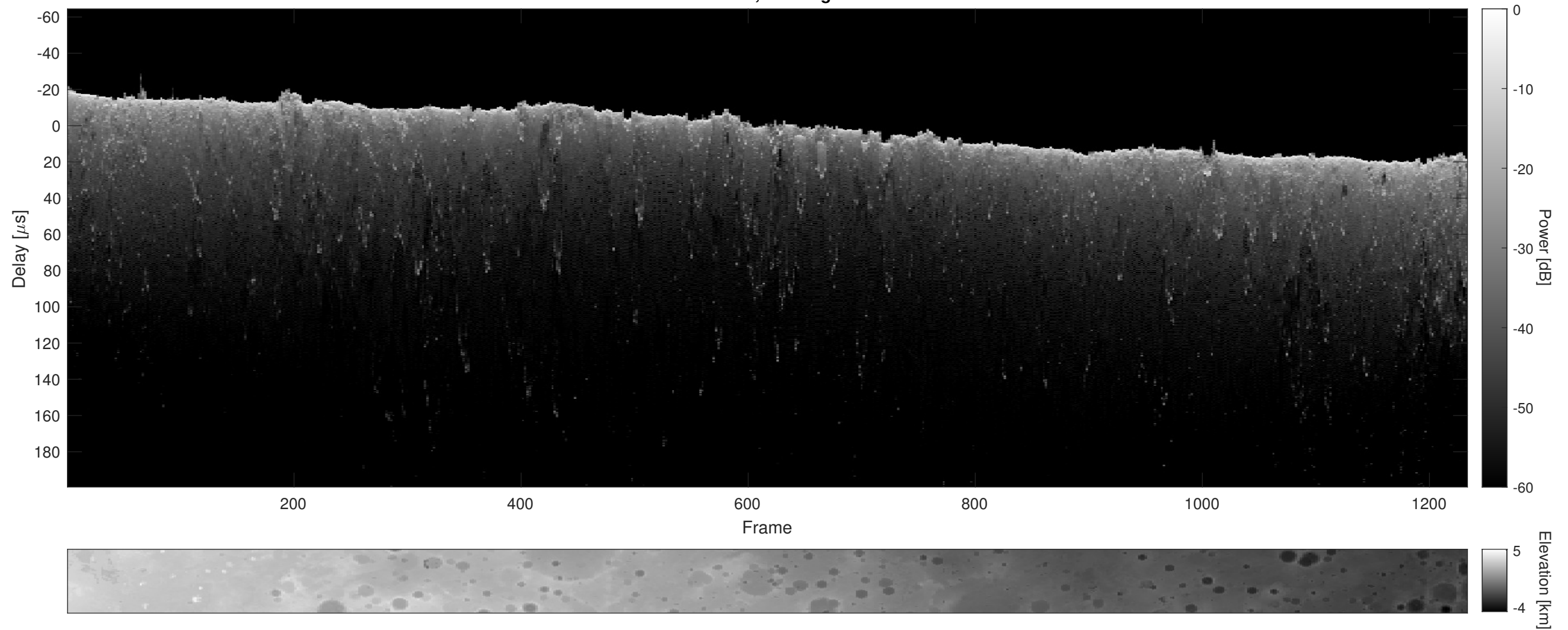
Orbit 4207, Cluttergram
