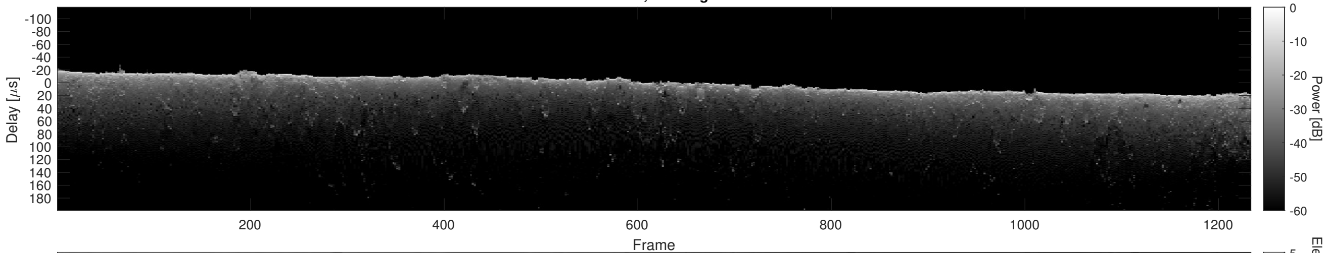
Orbit 4207, Cluttergram
