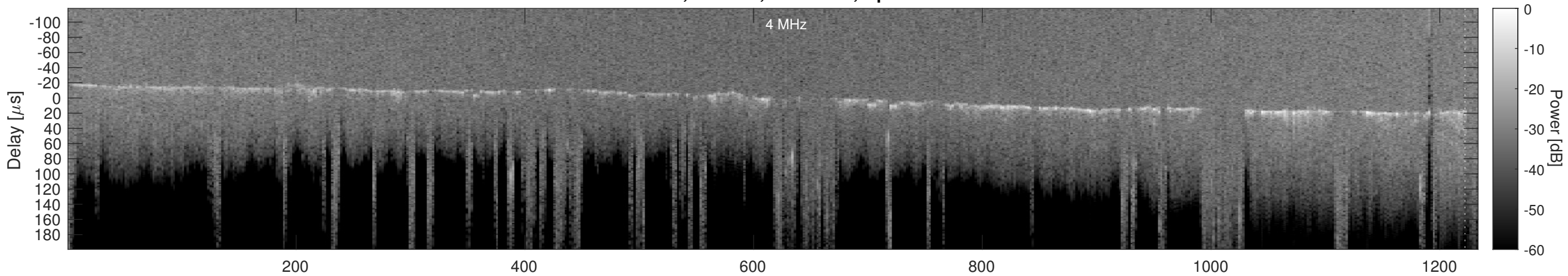
Orbit 4207, Cluttergram
