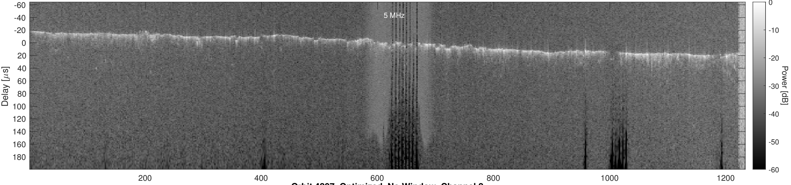
Orbit 4207, Optimized, No Window, Channel 2
