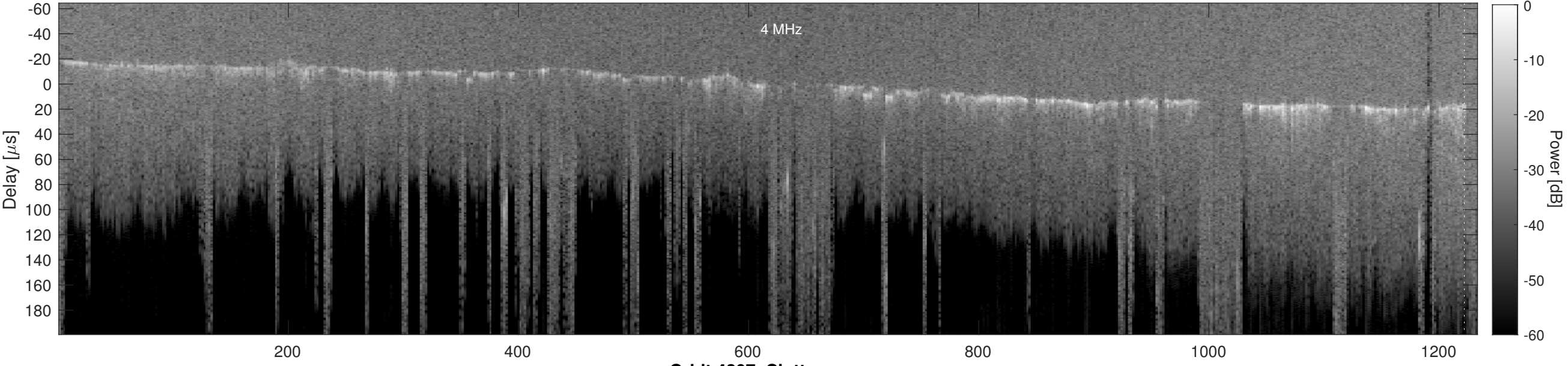
Orbit 4207, Cluttergram
