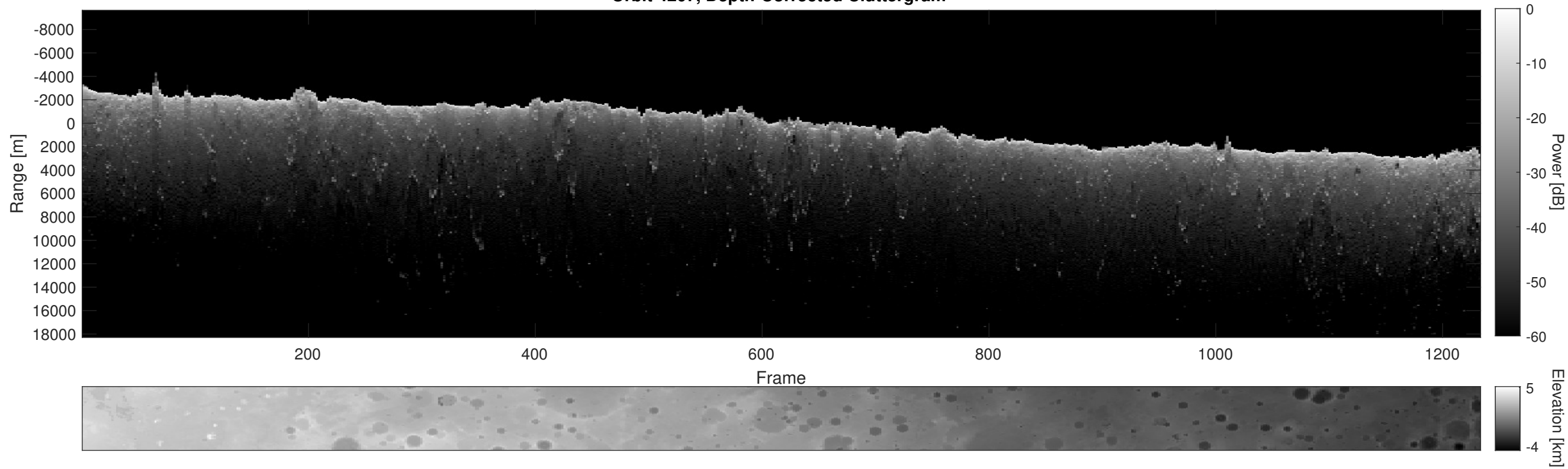
Orbit 4207, Depth-Corrected Cluttergram
