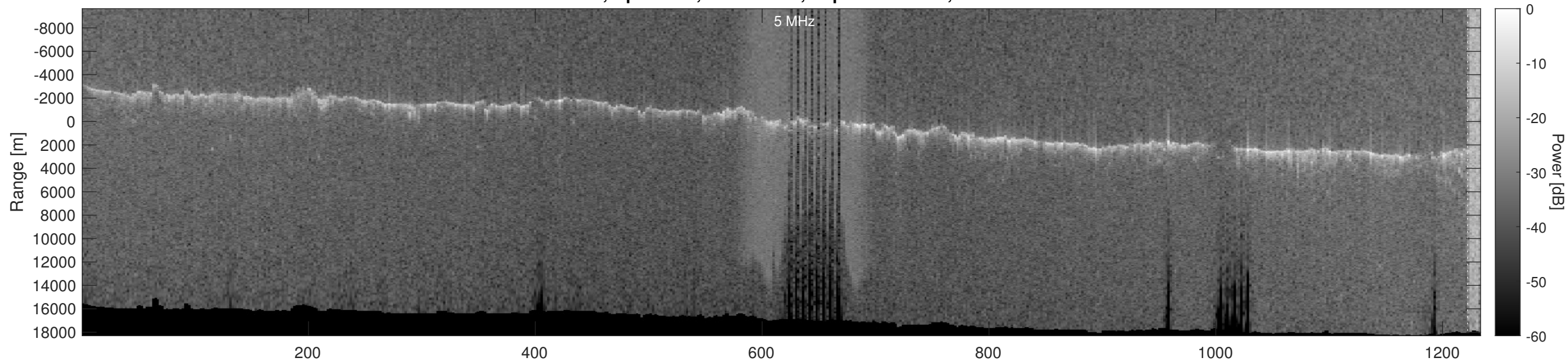
Orbit 4207, Optimized, No Window, Depth-Corrected, Channel 2
