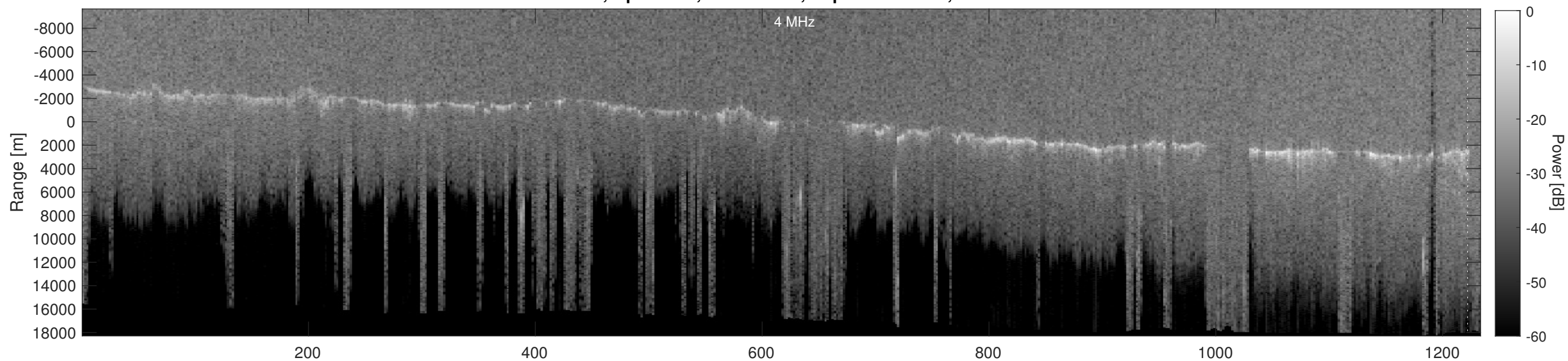
Orbit 4207, Depth-Corrected Cluttergram
