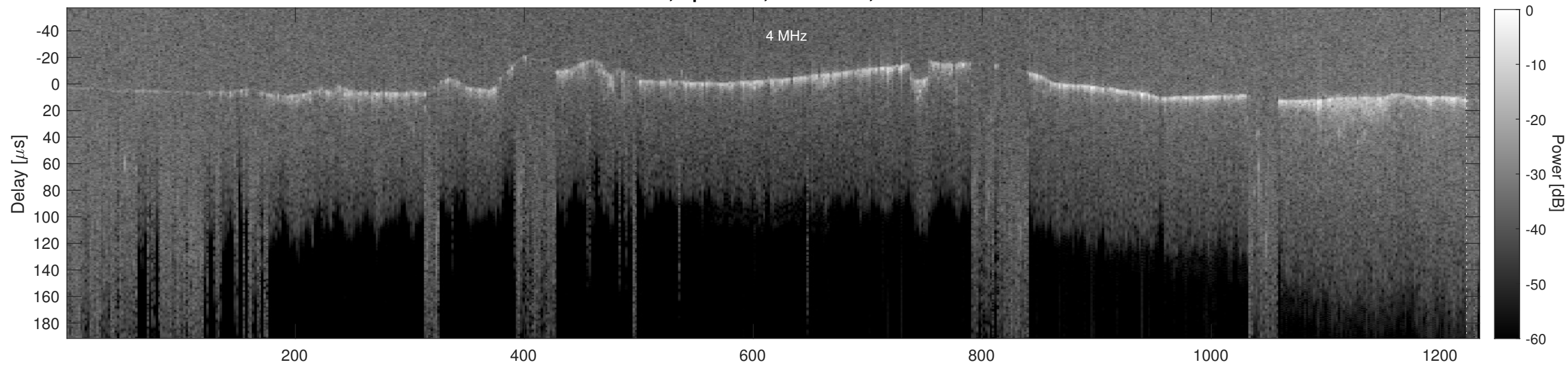
Orbit 4208, Cluttergram
