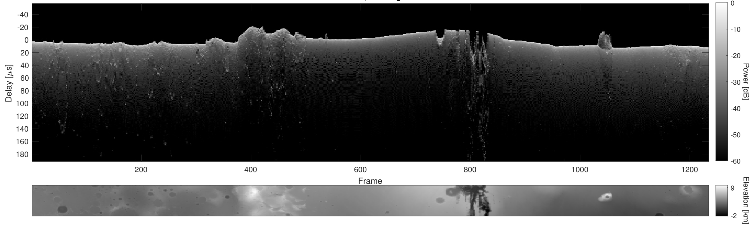
Orbit 4208, Cluttergram
