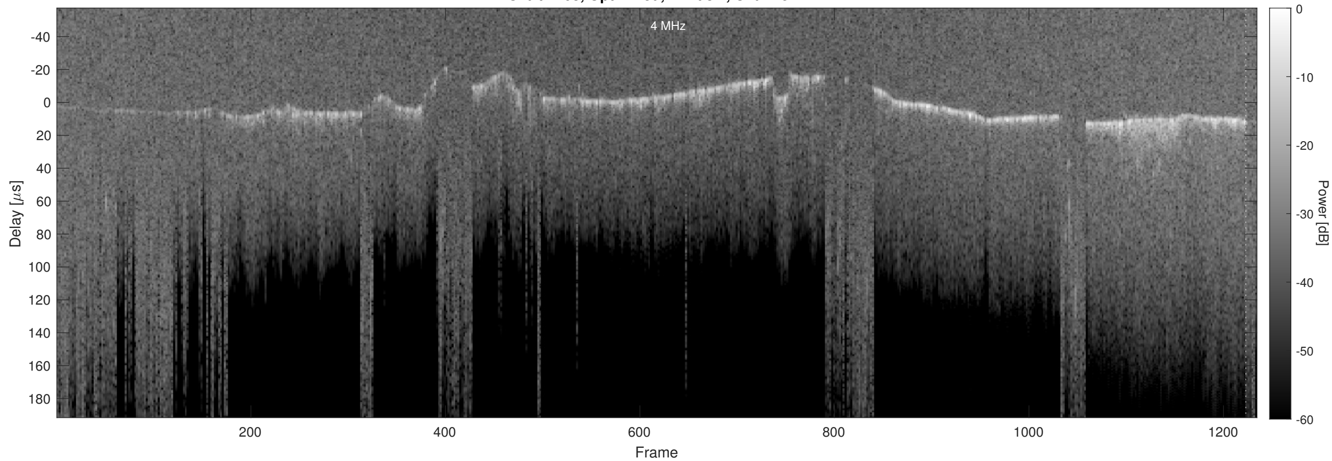
Orbit 4208, Optimized, Window, Channel 2
