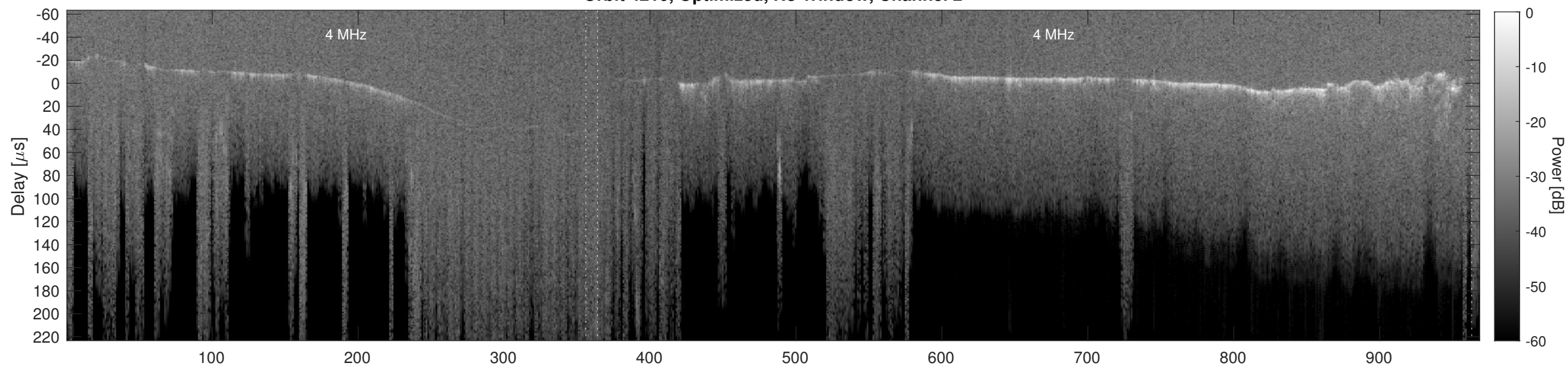
Orbit 4210, Cluttergram
