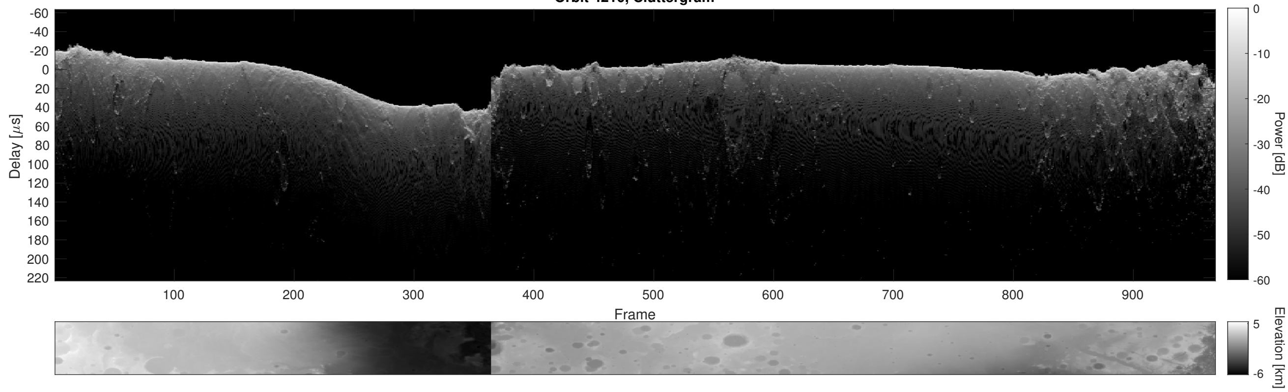
Orbit 4210, Cluttergram
