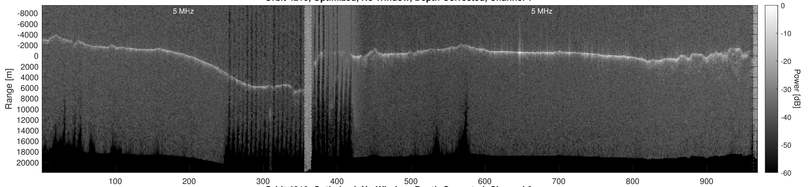
Orbit 4210, Optimized, No Window, Depth-Corrected, Channel 2
