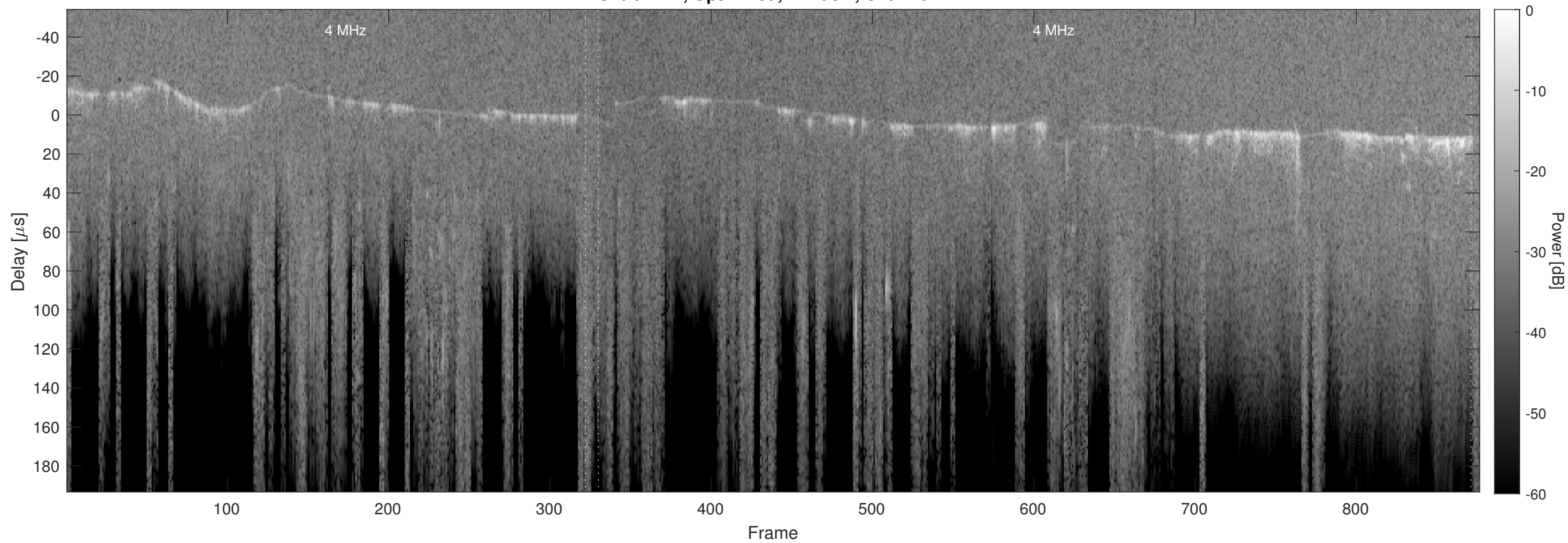
Orbit 4214, Optimized, Window, Channel 2
