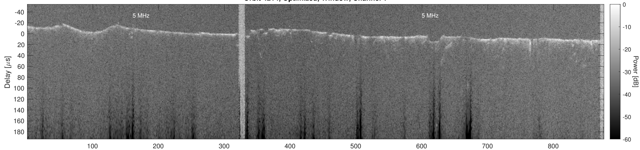
Orbit 4214, Optimized, Window, Channel 2
