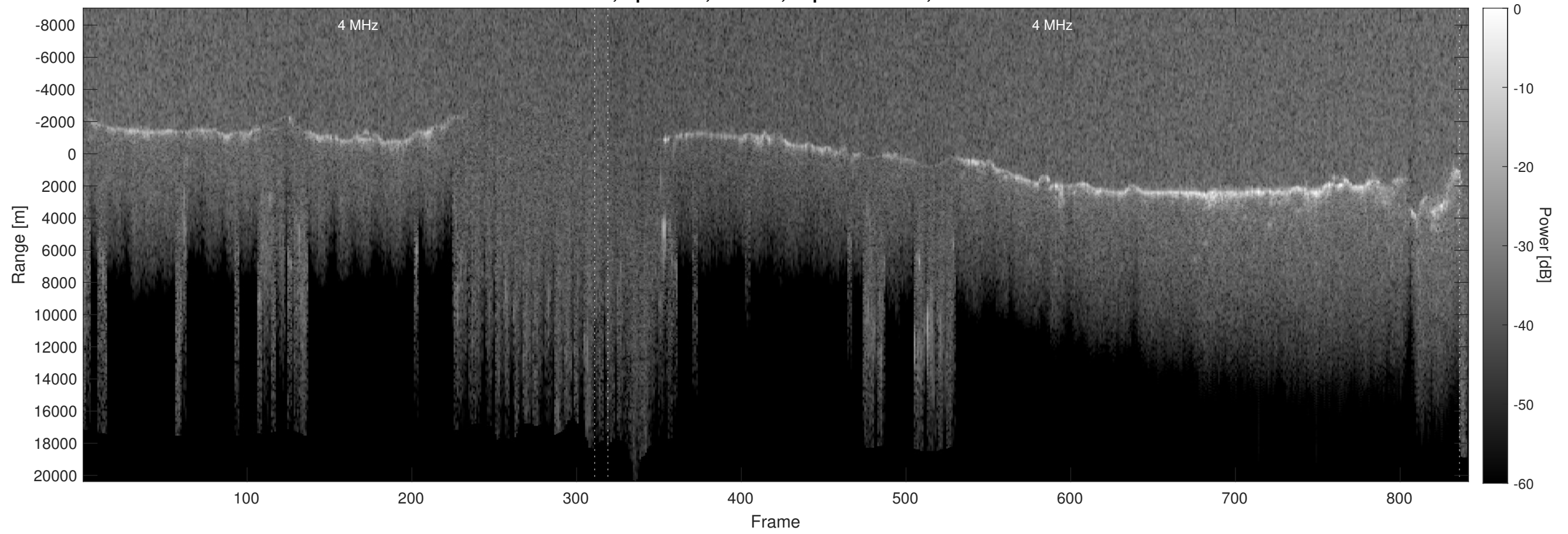
Orbit 4215, Optimized, Window, Depth-Corrected, Channel 2
