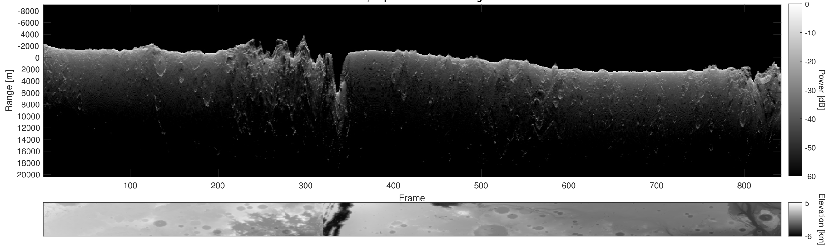
Orbit 4215, Depth-Corrected Cluttergram
