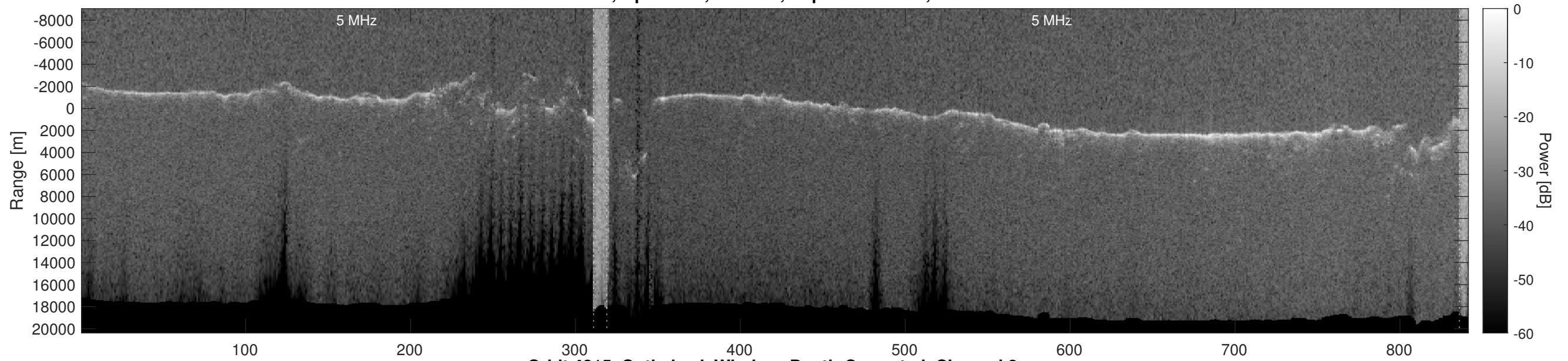
Orbit 4215, Optimized, Window, Depth-Corrected, Channel 2
