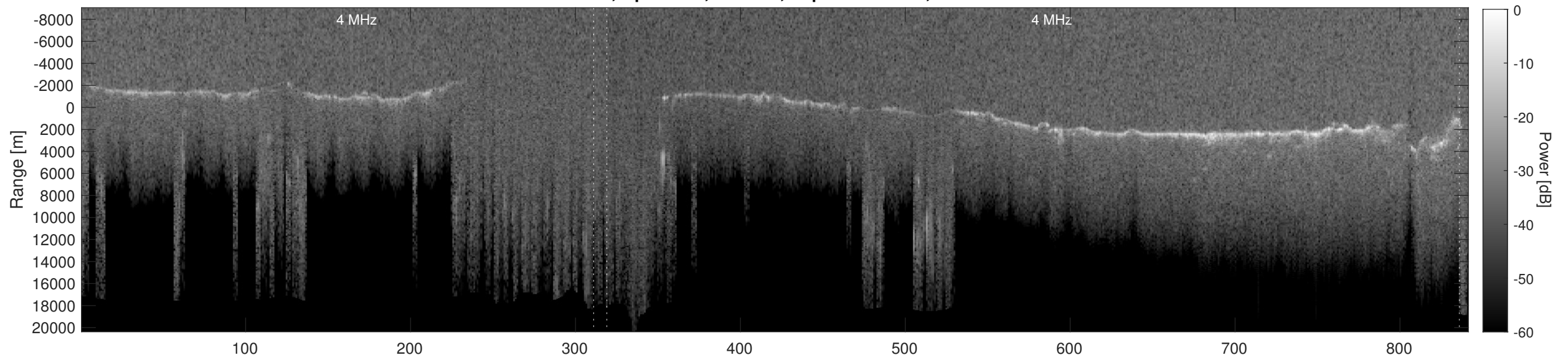
Orbit 4215, Depth-Corrected Cluttergram
