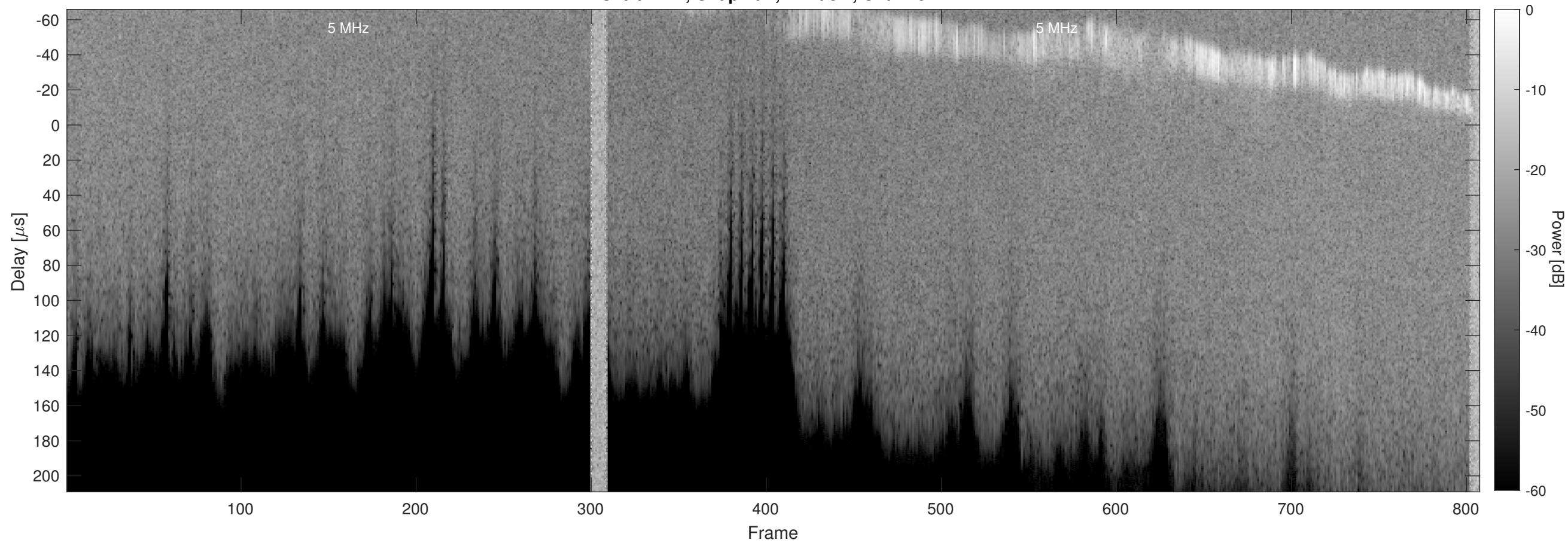
Orbit 4217, Chapman, Window, Channel 2
