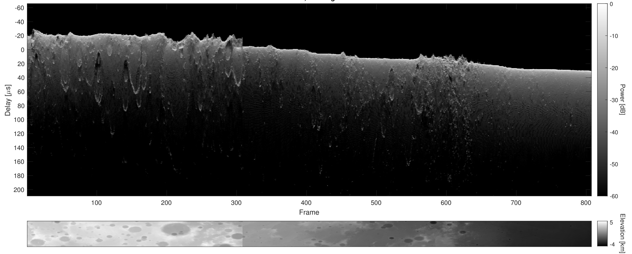
Orbit 4217, Cluttergram
