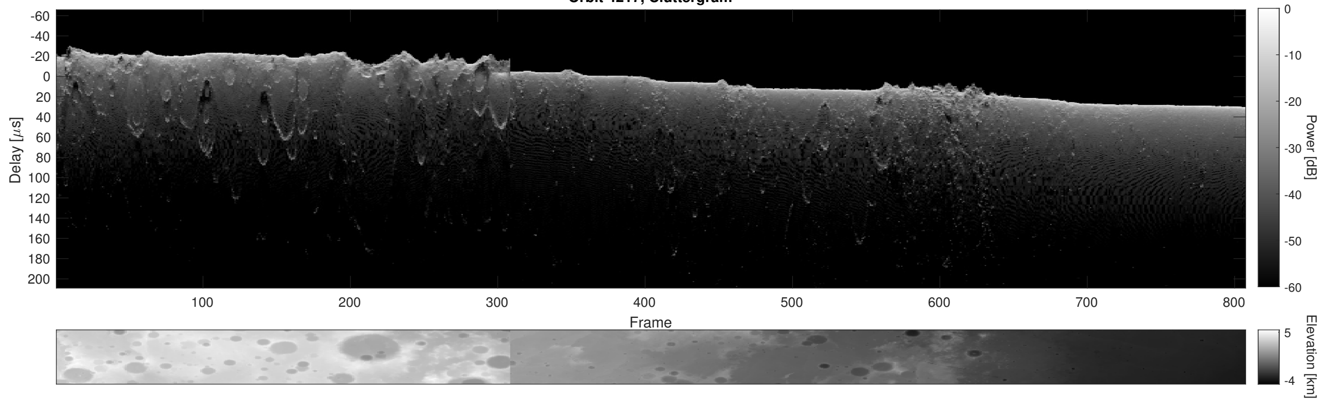
Orbit 4217, Cluttergram
