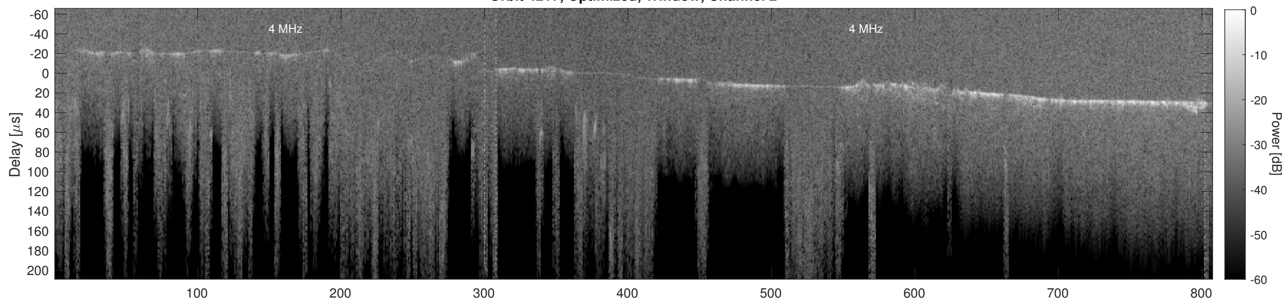
Orbit 4217, Cluttergram
