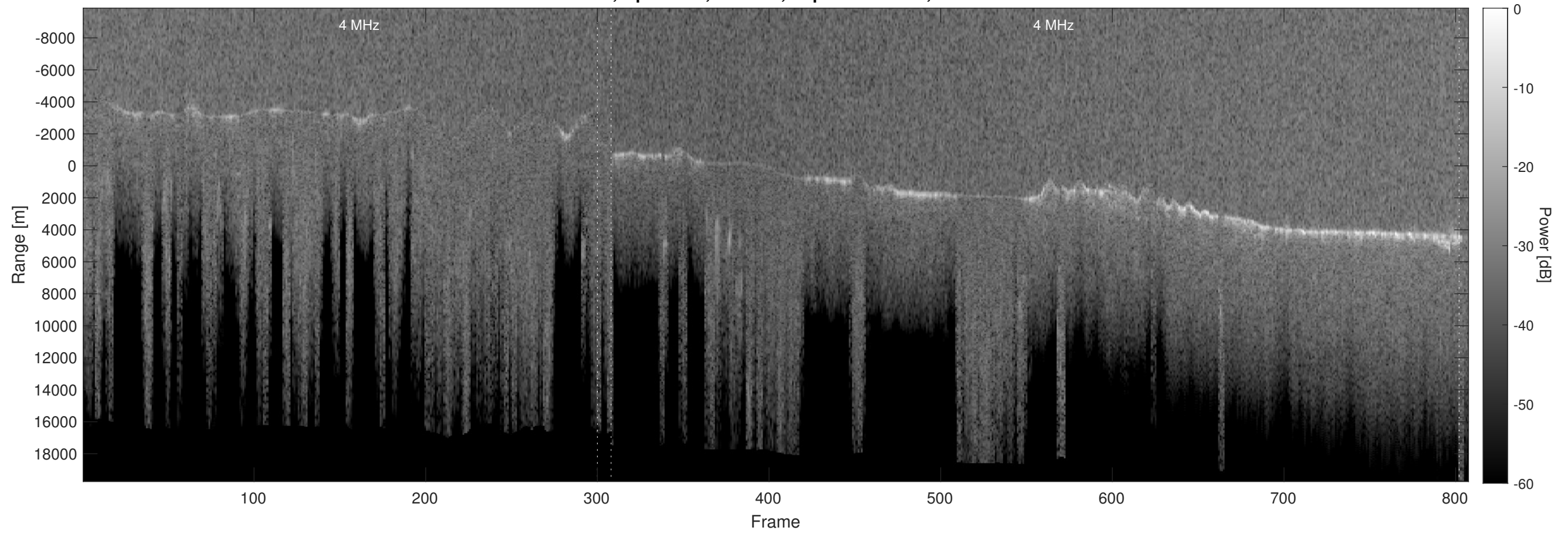
Orbit 4217, Optimized, Window, Depth-Corrected, Channel 2
