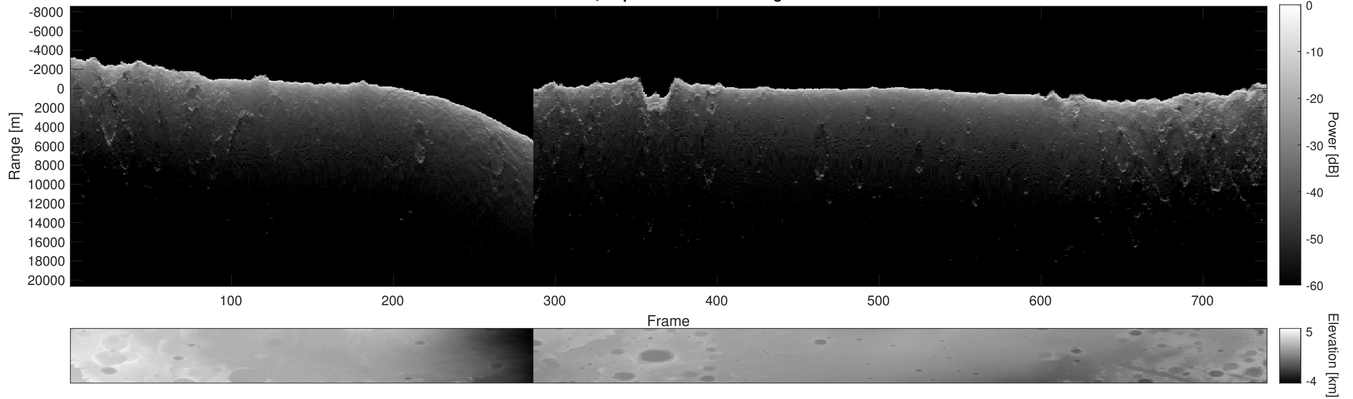
Orbit 4221, Depth-Corrected Cluttergram
