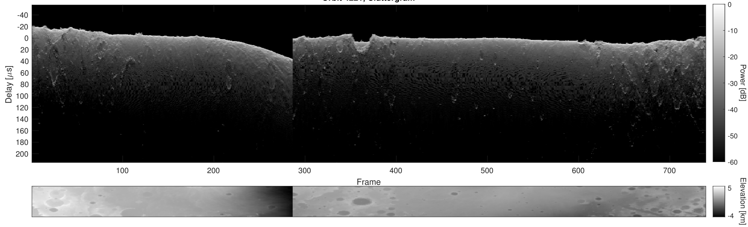
Orbit 4221, Cluttergram
