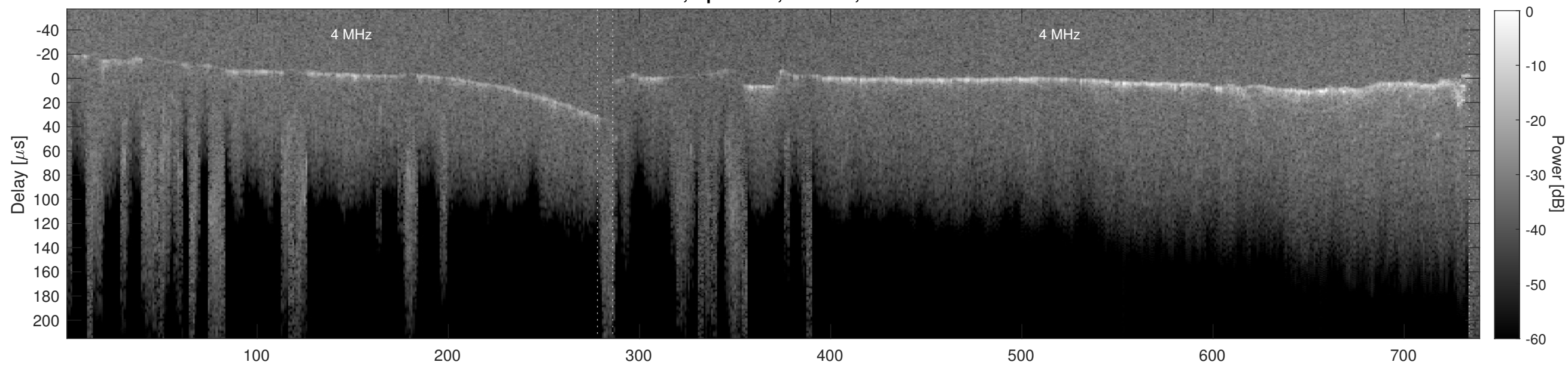
Orbit 4221, Cluttergram
