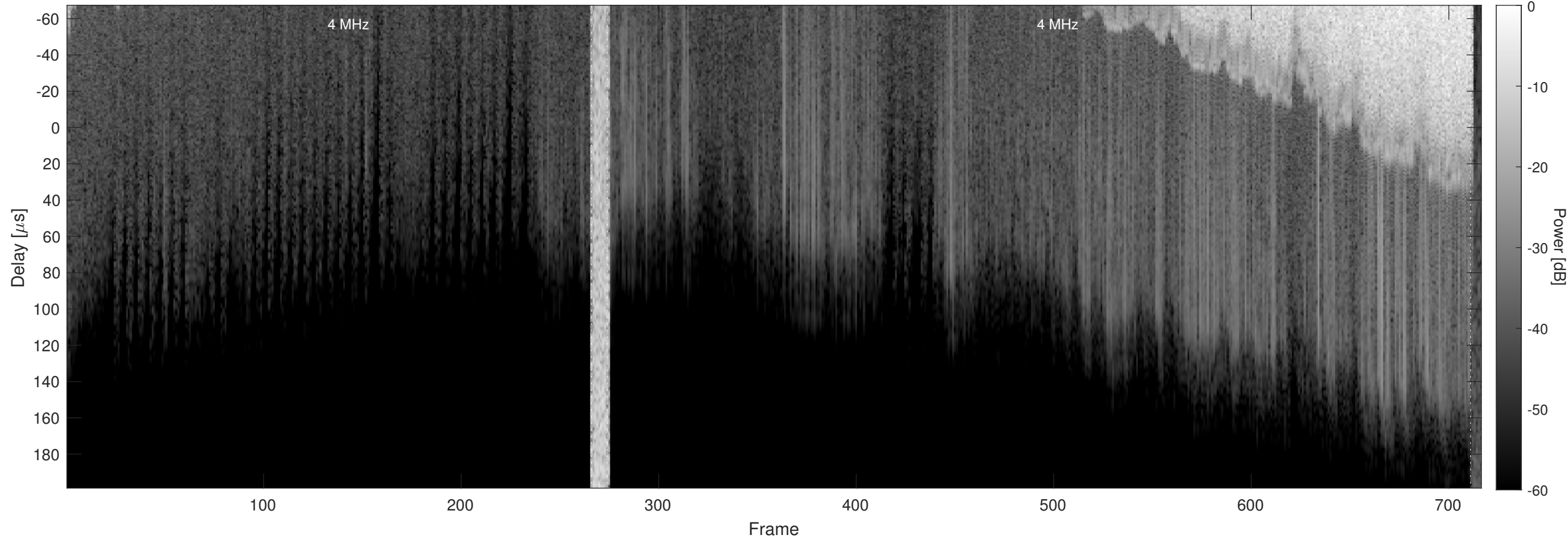
Orbit 4223, Chapman, No Window, Channel 2
