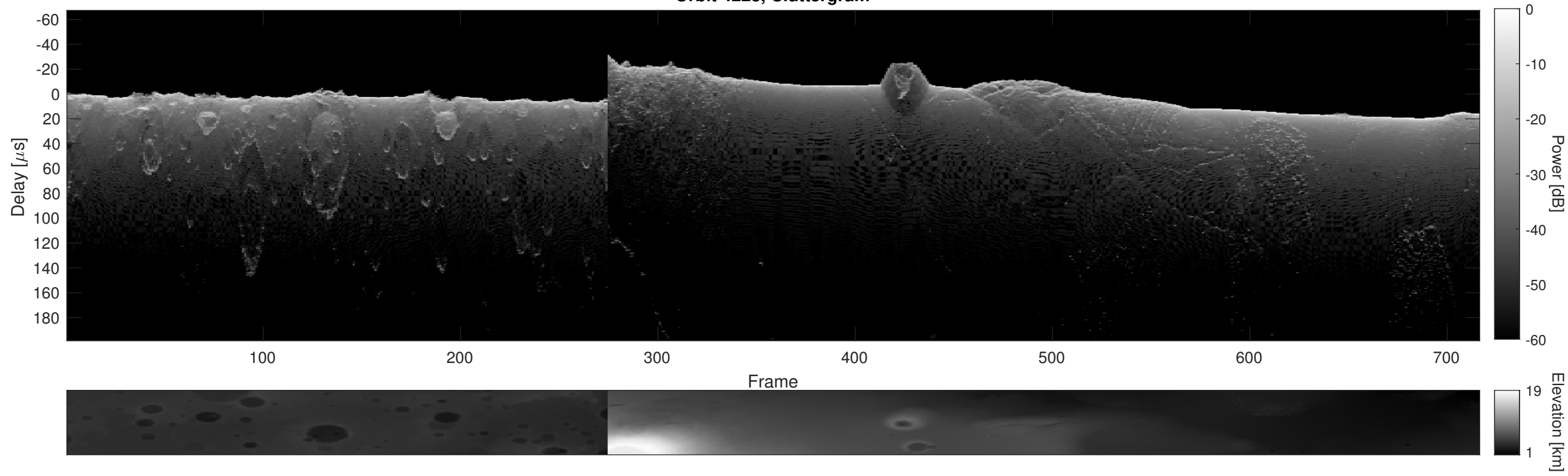
Orbit 4223, Cluttergram
