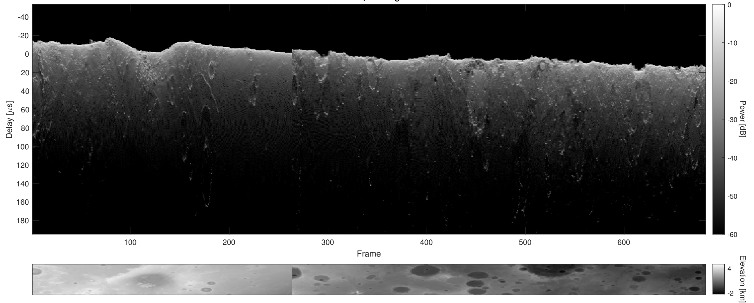
Orbit 4225, Cluttergram
