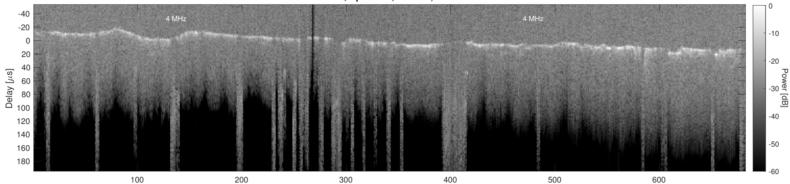
Orbit 4225, Cluttergram
