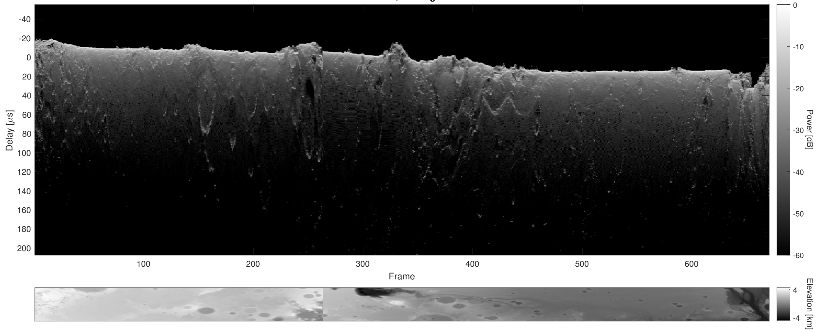
Orbit 4226, Cluttergram
