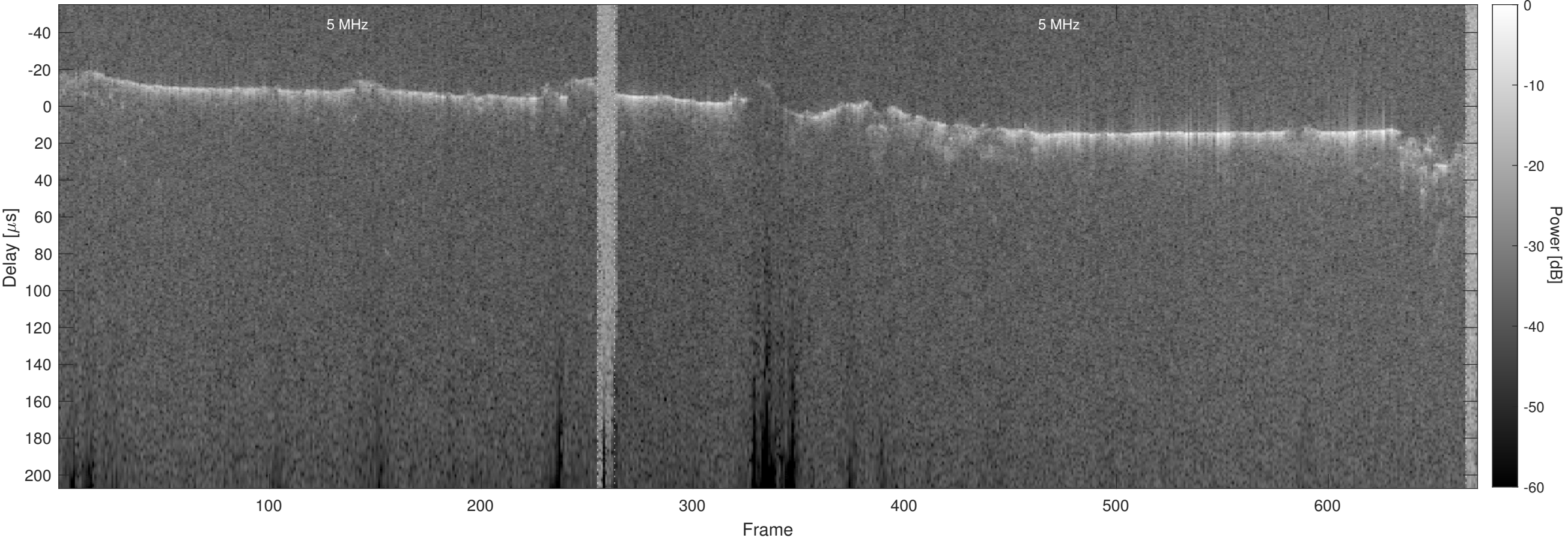
Orbit 4226, Optimized, No Window, Channel 2
