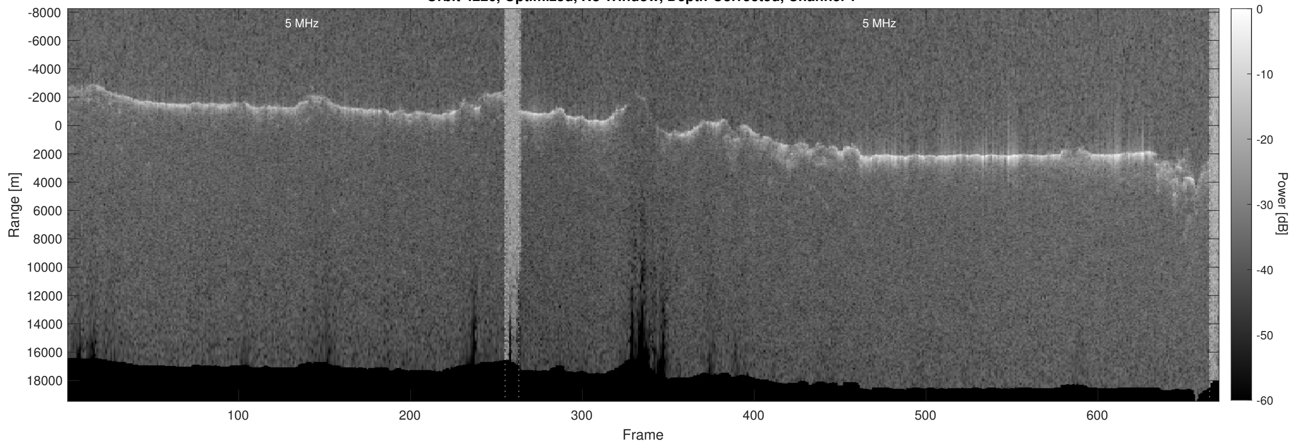
Orbit 4226, Optimized, No Window, Depth-Corrected, Channel 2
