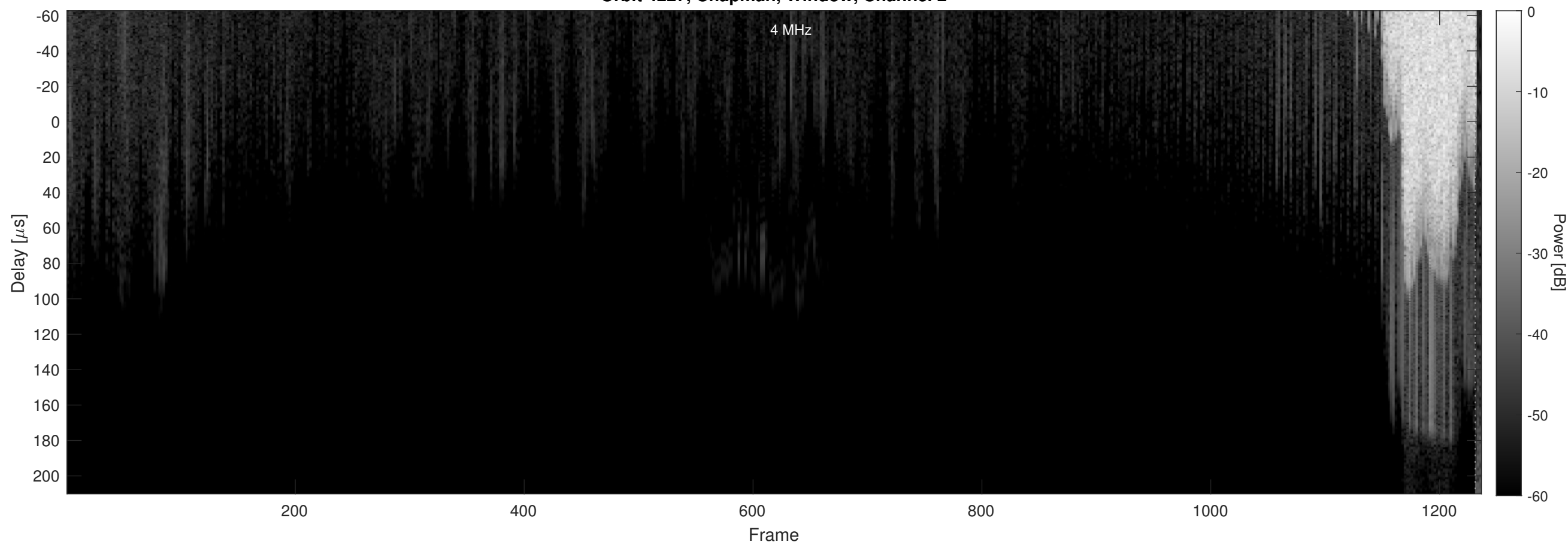
Orbit 4227, Chapman, Window, Channel 2
