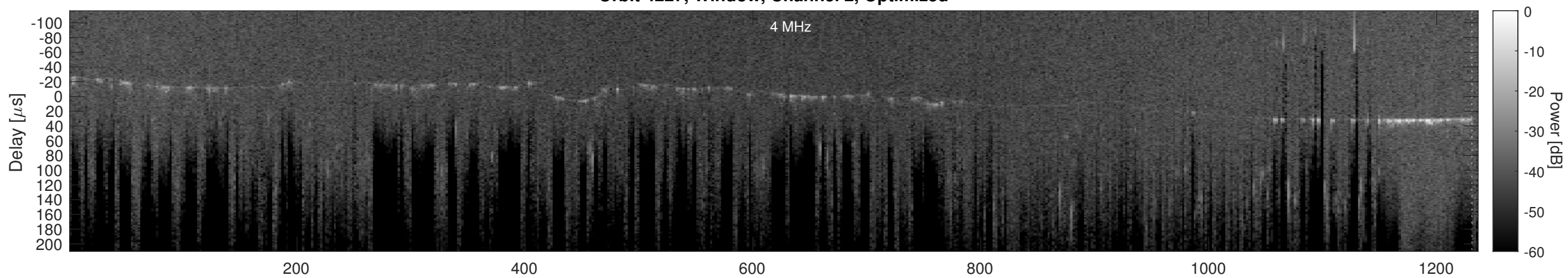
Orbit 4227, Cluttergram
