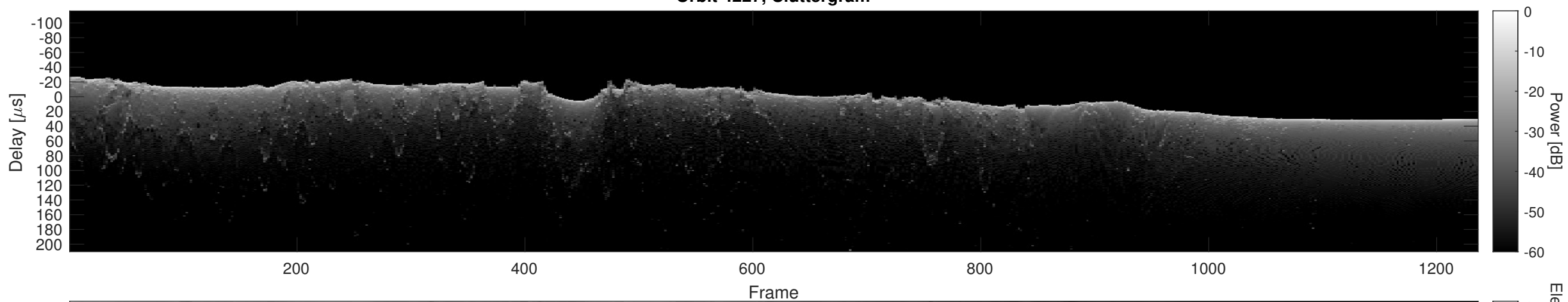
Orbit 4227, Cluttergram
