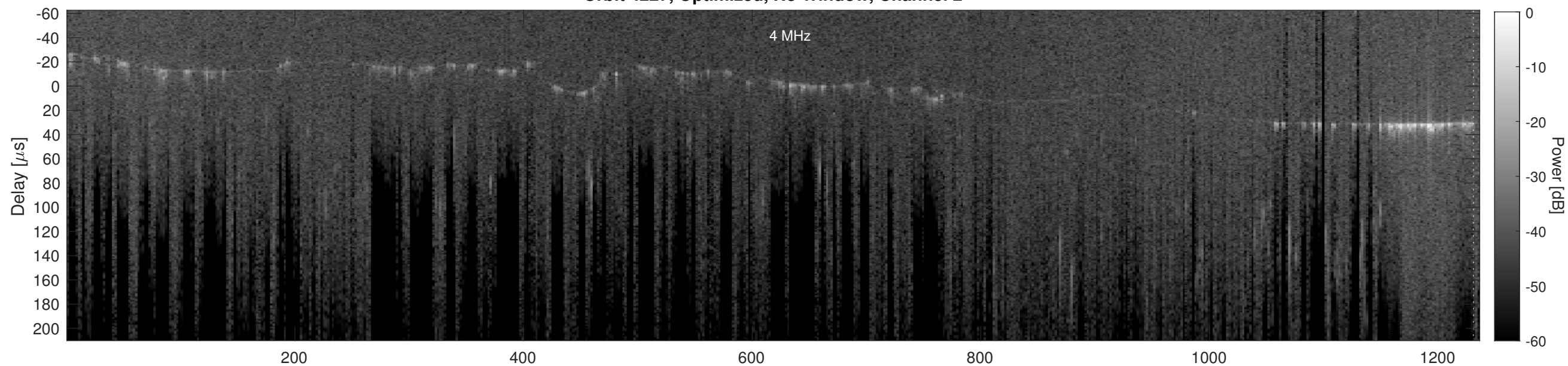
Orbit 4227, Cluttergram
