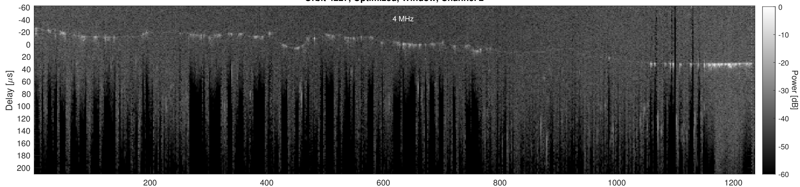
Orbit 4227, Cluttergram
