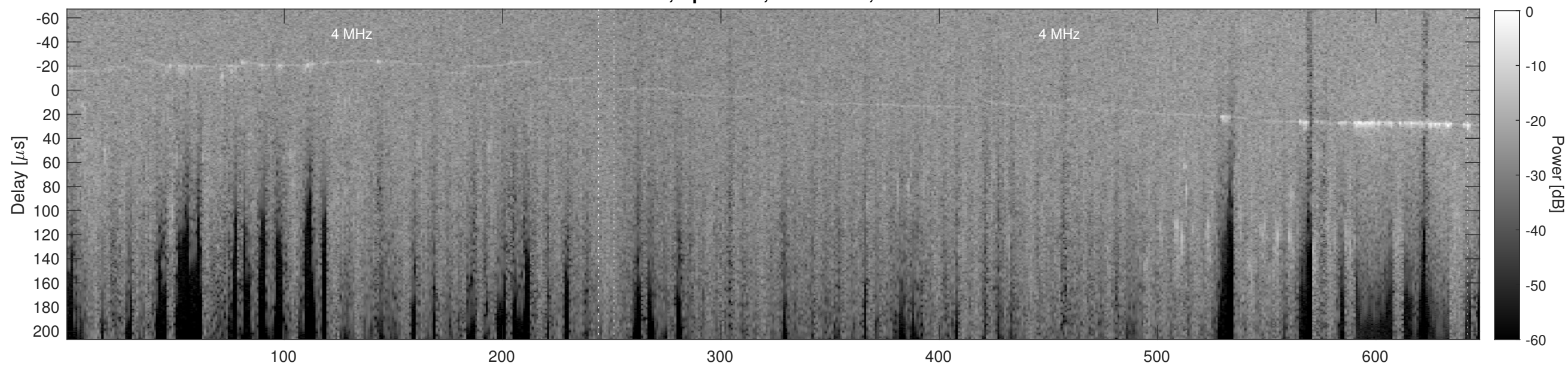
Orbit 4228, Cluttergram
