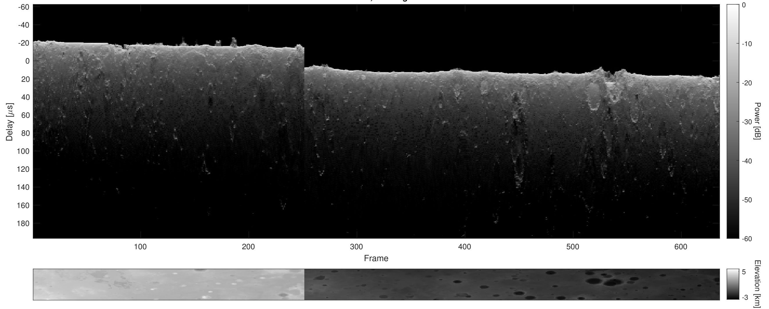
Orbit 4229, Cluttergram
