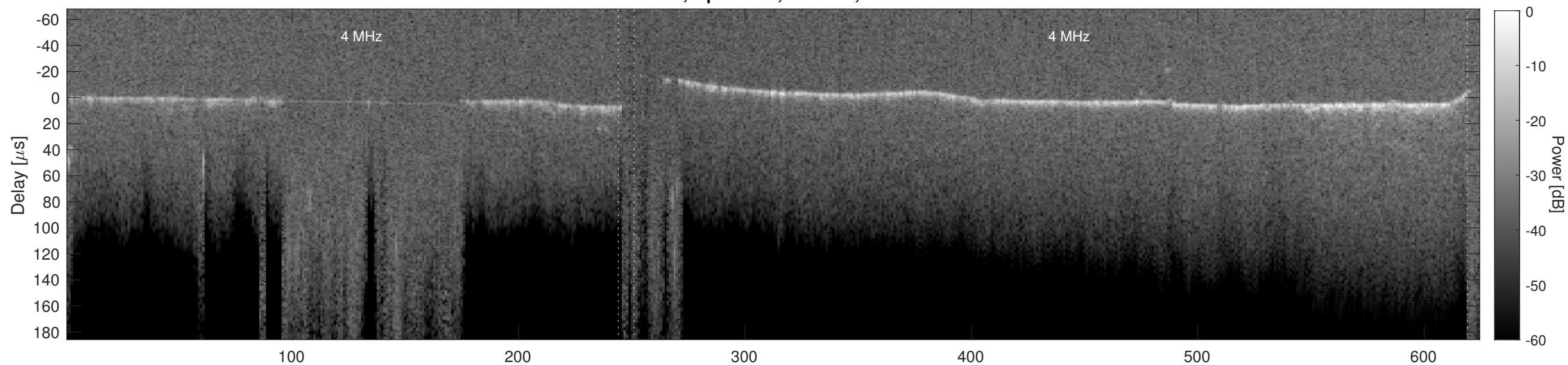
Orbit 4230, Cluttergram
