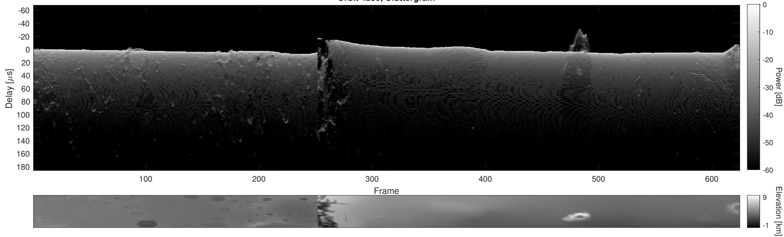
Orbit 4230, Cluttergram
