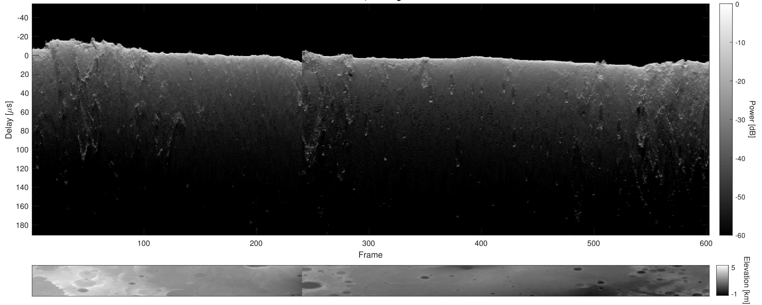
Orbit 4232, Cluttergram
