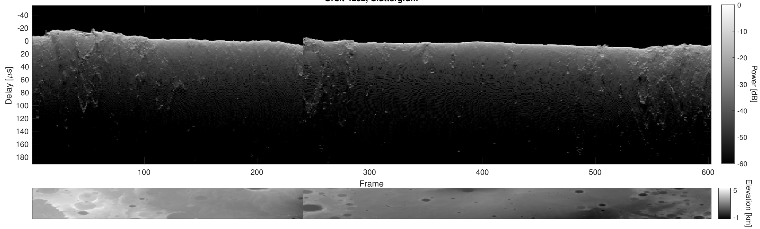
Orbit 4232, Cluttergram
