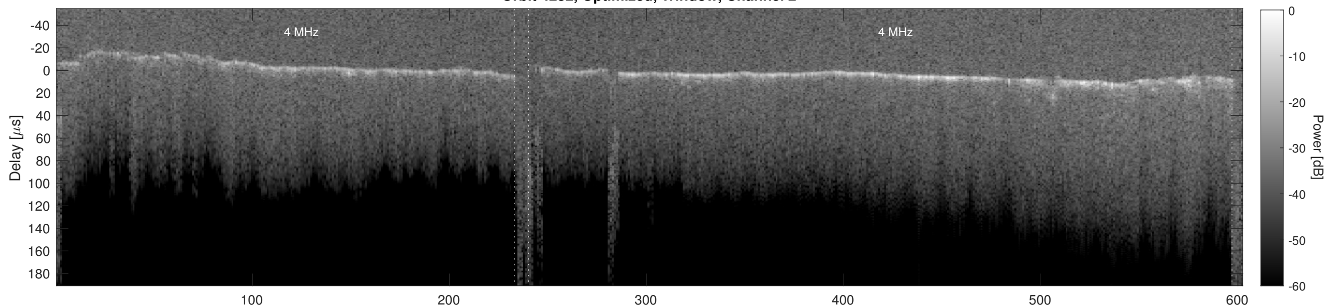
Orbit 4232, Cluttergram
