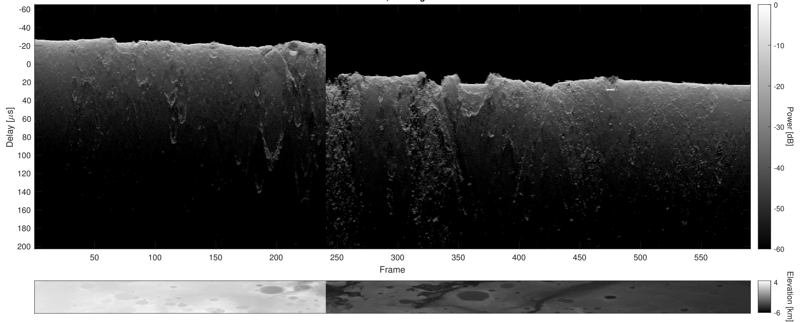
Orbit 4233, Cluttergram
