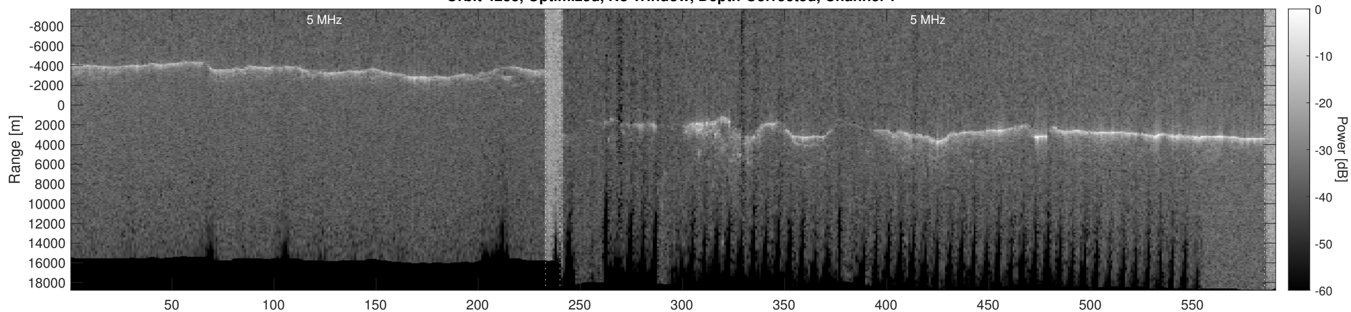
Orbit 4233, Optimized, No Window, Depth-Corrected, Channel 2
