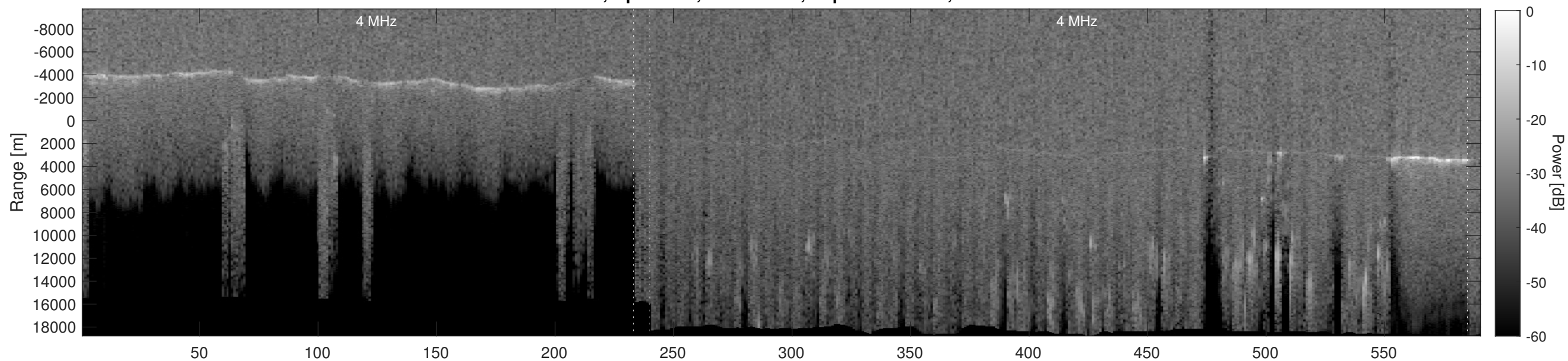
Orbit 4233, Depth-Corrected Cluttergram
