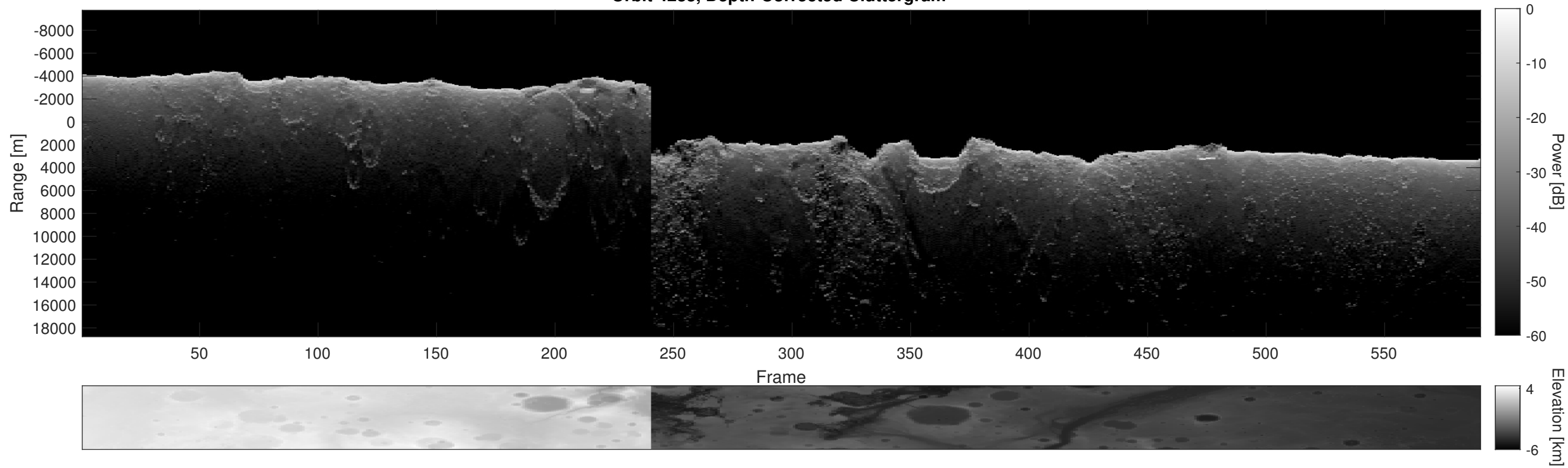
Orbit 4233, Depth-Corrected Cluttergram
