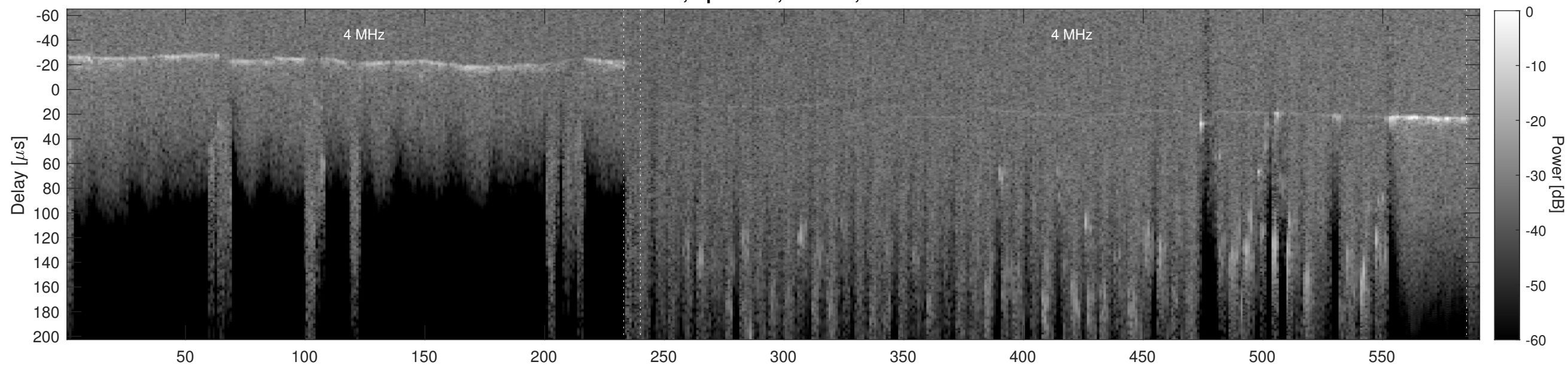
Orbit 4233, Cluttergram
