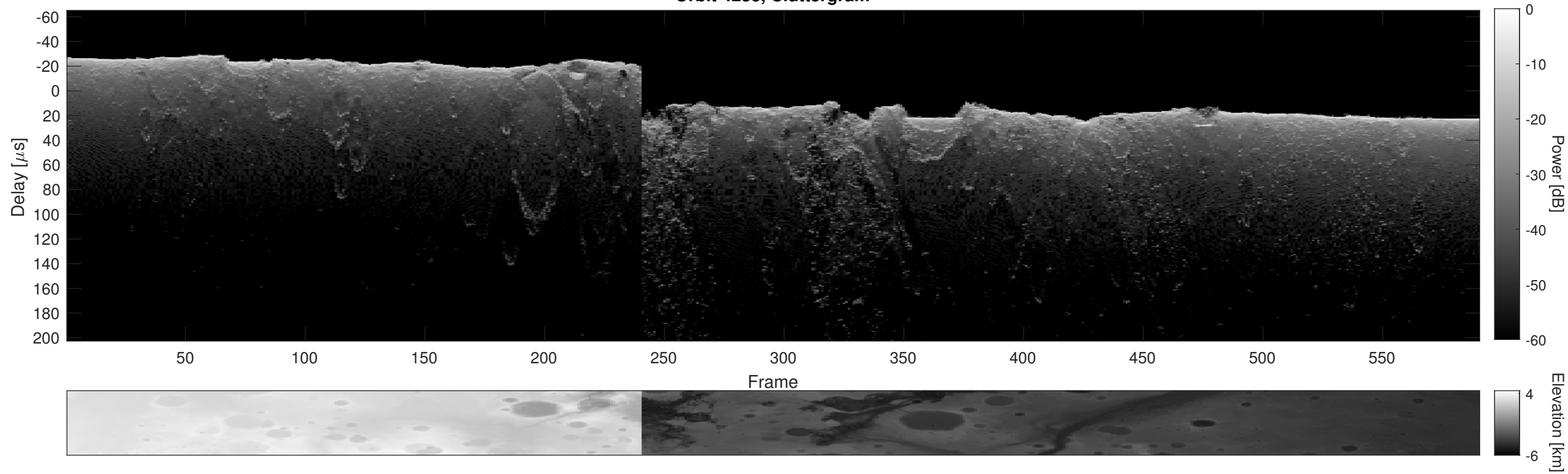
Orbit 4233, Cluttergram
