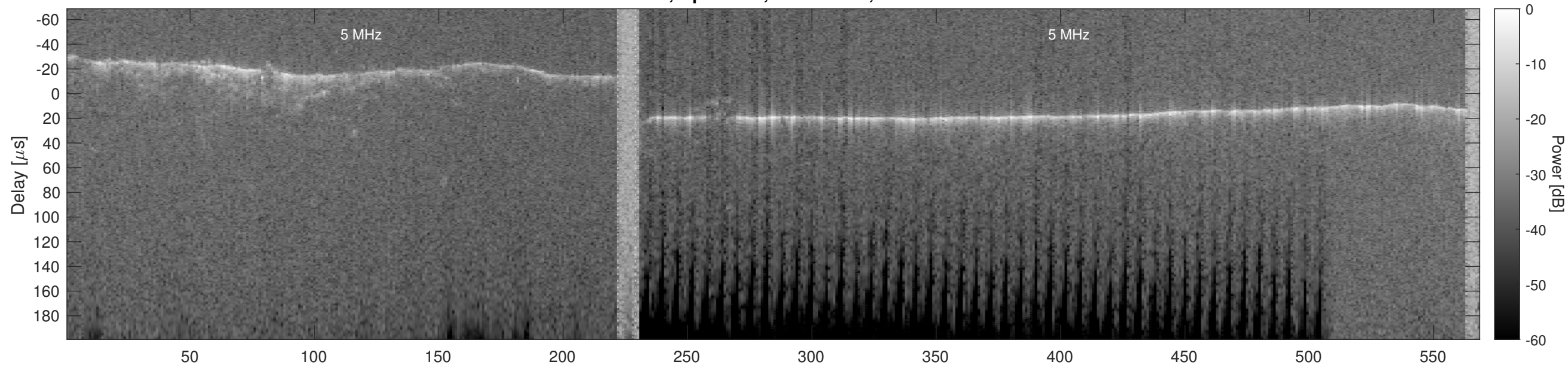
Orbit 4235, Optimized, No Window, Channel 2
