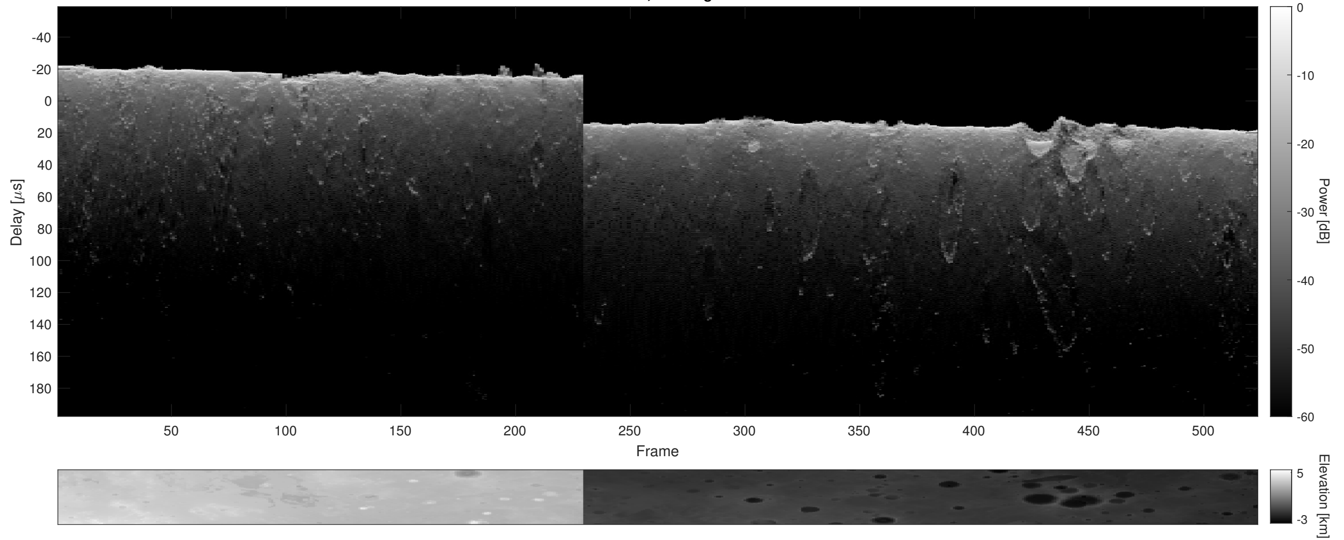
Orbit 4240, Cluttergram
