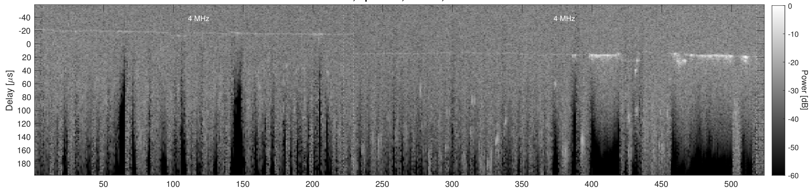
Orbit 4240, Cluttergram
