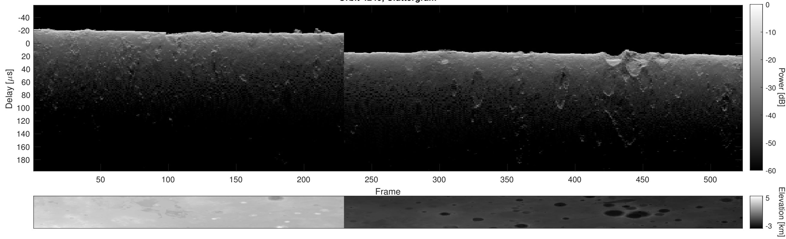
Orbit 4240, Cluttergram
