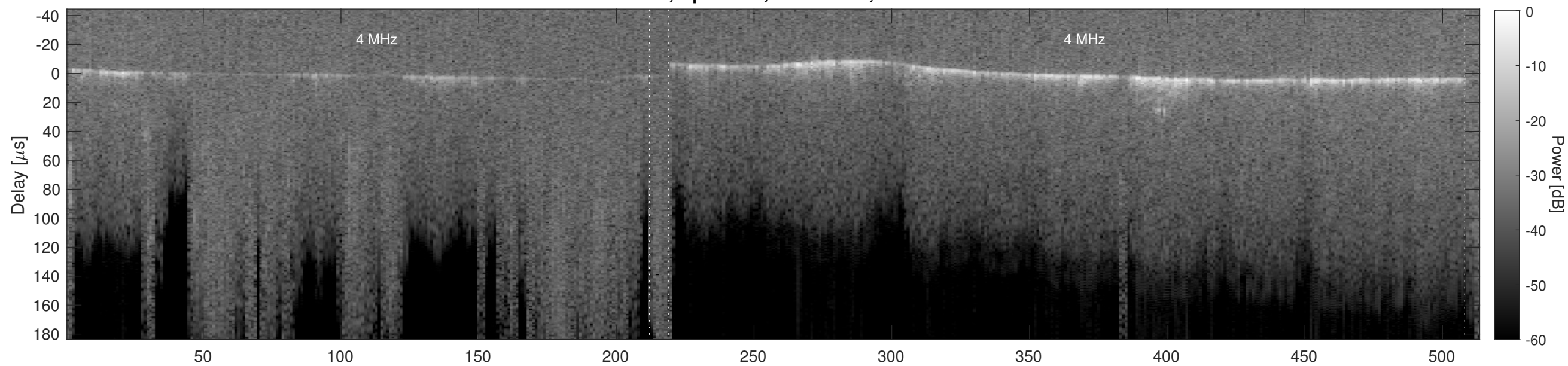
Orbit 4241, Cluttergram
