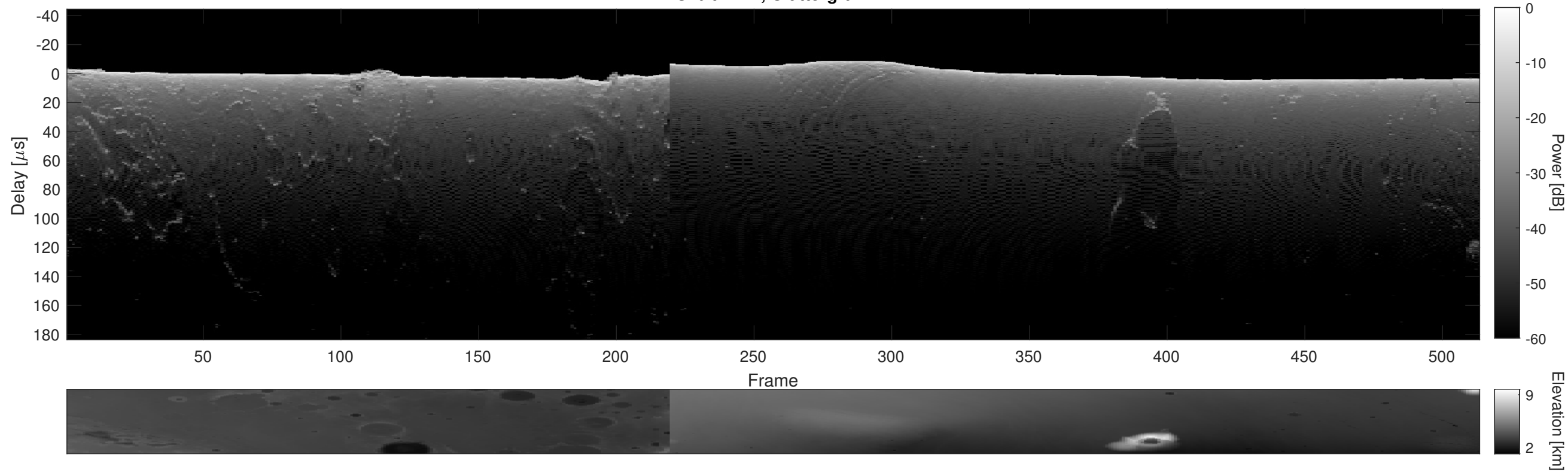
Orbit 4241, Cluttergram
